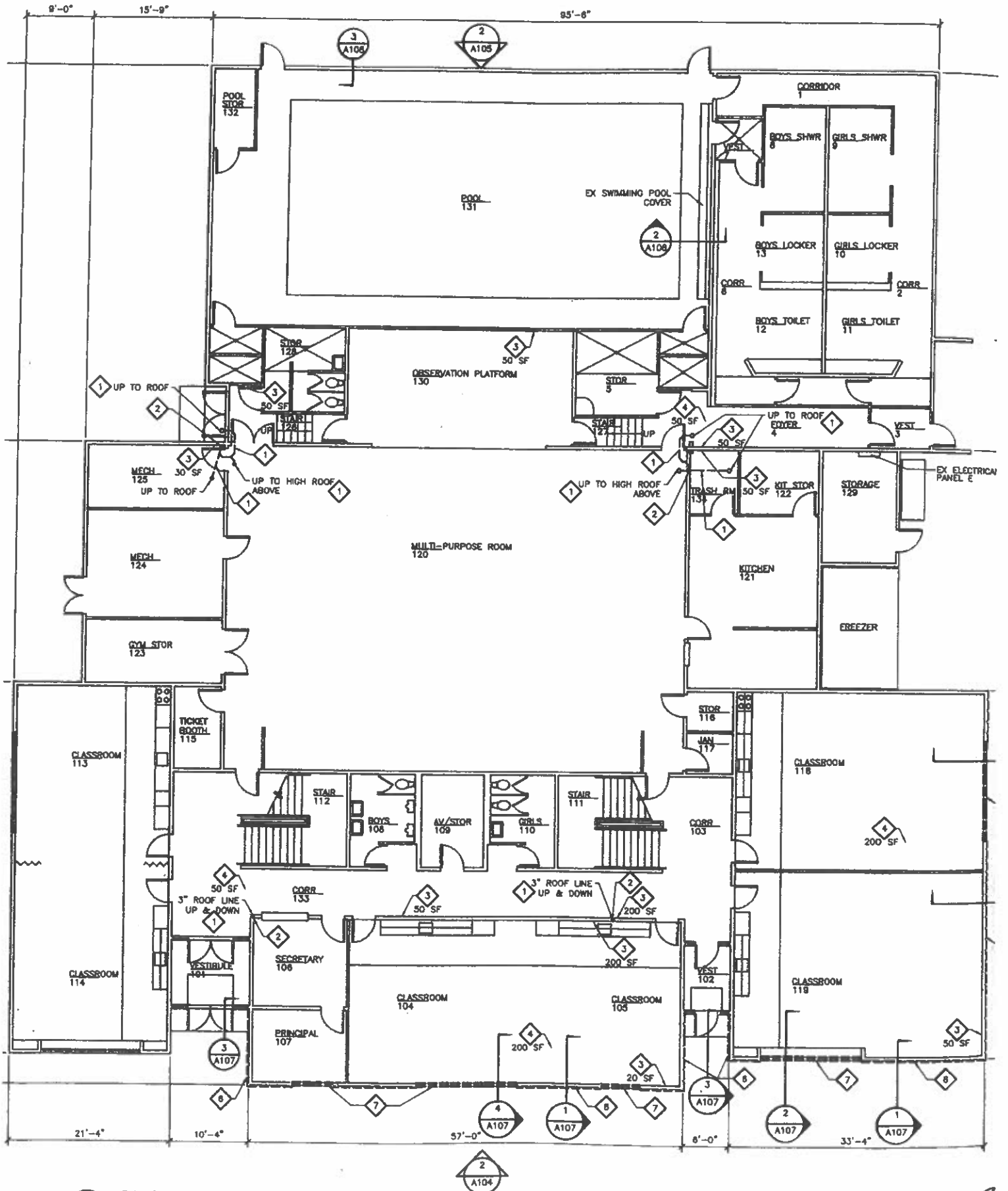
1 FIRST FLOOR DEMOLITION PLAN
